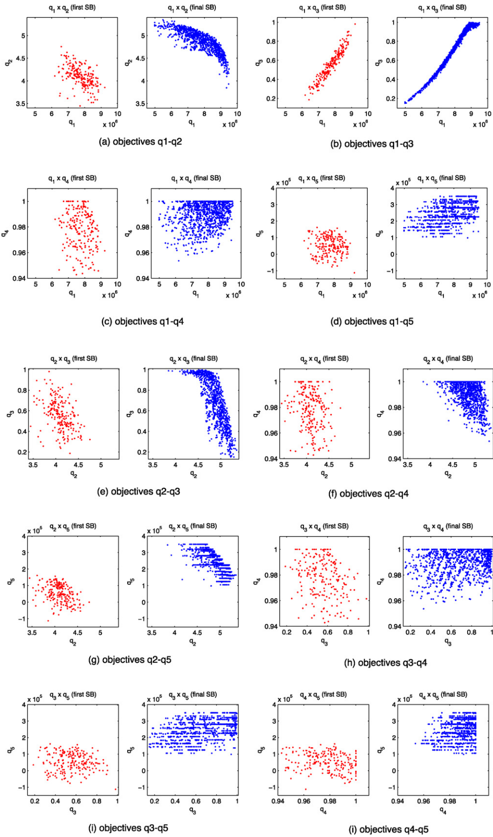
Fig. 1. Illustration of an improvement of the final solution base w.r.t. the initial solution base. For the sake of easy visualization 2D projections of the non-dominated solutions are shown in a couple of separate plots – the left one for the initial solution base and the right one for the final solution base – for all pairs of objectives.
